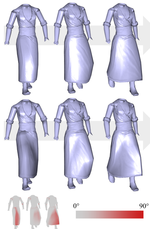
Figure 1: Lighting a skinned low-poly, normal-mapped model. Top sequence: the standard method produces inaccurate normals that makes the skirt look flat. Mid sequence: our algorithm produces an accurate lighting which better conveys the shape of the skirt. Bottom: differences in normals. See also attached video.
